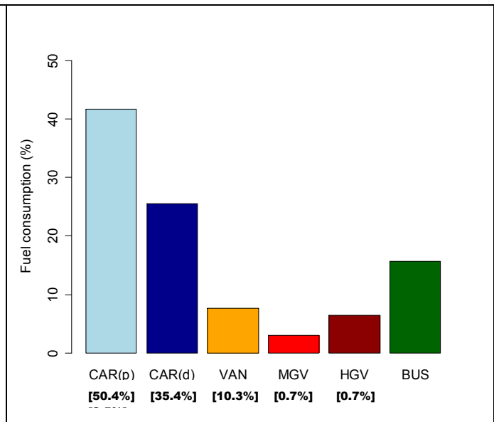
FIGURE 2: Fuel consumption
